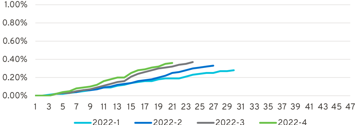
2022 Transactions
