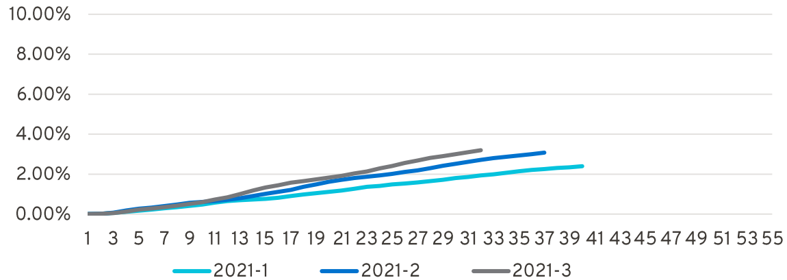
2021 Transactions
