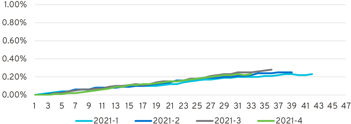
2021 Transactions
